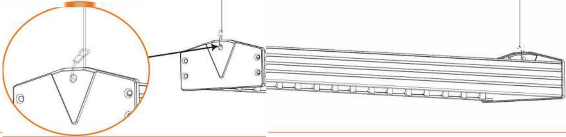
Suspended mounted
