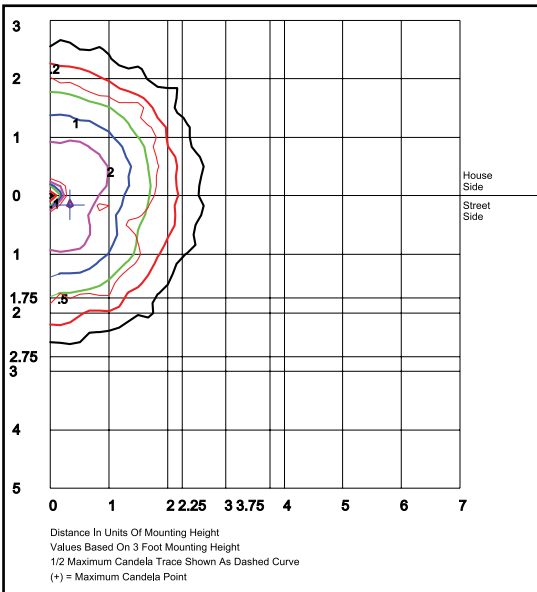
NIKLAS 5-1X14-U-AM 360° Open - Clear Glass Lens Grid in feet, Mounting Height = 3 ft.
