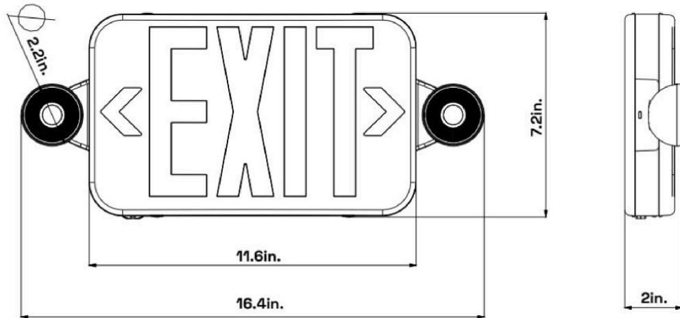
RENZO EMERGENCY / EXIT COMBO — FRONT AND SIDE ELEVATION. SIGN BODY 11.60" WIDE; EACH HEAD Ø2.20".
