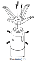
SF3 3" Tenon Φ76mm
