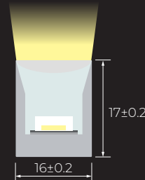
Cross Section(mm)
