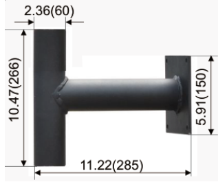
WL Wall Mount Bracket arm
