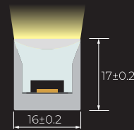
Cross Section(mm)
