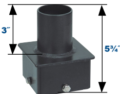
5" Single Square Vertical Tenon - 2 3/8" Dia. PSS53SVTZ
