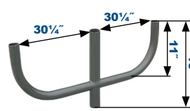
180° Triple Bullhorn PRSTR180BHZ Wt lbs 27, EPA 1.5
