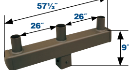
5" Triple Square Vertical Tenon PSS5TRVTZ Wt lbs 46, EPA 1.9
