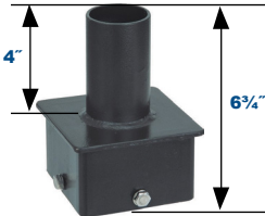
4" Single Square Vertical Tenon - 2 3/4" Dia. PSS42SVTZ
