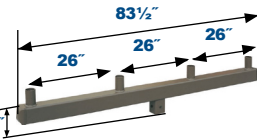
4" 180° Quad Square Vertical Tenon PSS4Q180VTZ Wt lbs 56, EPA 2.7
