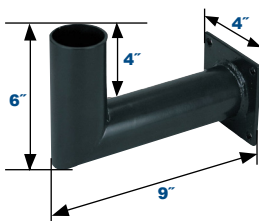
Wall Mount 90° Bracket PRSWMB90Z
