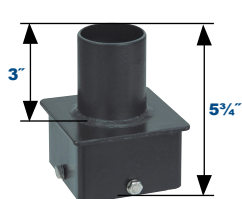
4" Single Square Vertical Tenon - 2 1/2" Dia. PSS43SVTZ
