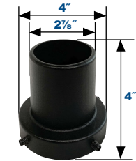
Retrofit Tenon Adaptor for 2 3/8" Tenons PSRTNB
