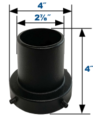
Retrofit Tenon Adaptor for 2 1/2" Tenons PSRTNB
