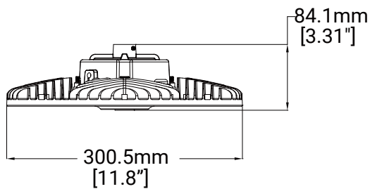
100W/150W
