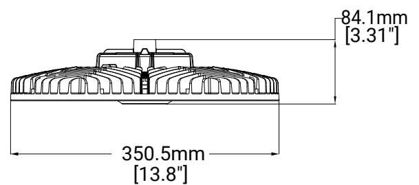
200W/240W/255W
