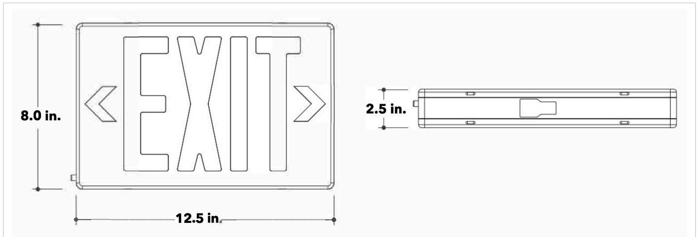
BENTO WET-LOCATION COMPACT EXIT SIGN — FRONT ELEVATION AND TOP VIEW.
