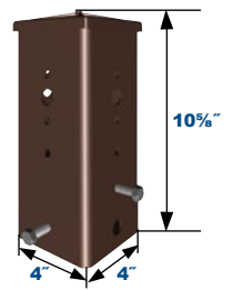
Pole Tenon Adaptor PTASUNVZ
