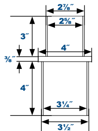
2 1/2" Single Round Vertical Tenon (P3) PSRA43B
