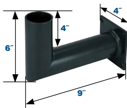
Wall Mount 90° Bracket PRSWMB90Z Wt lbs 4.5, EPA 0.3
