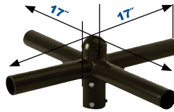
Quad Spoke Bracket, 90° Arms PTSB490SZ*
