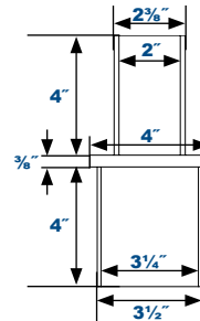
2 1/2" Single Round Vertical Tenon (P2) PSRA42B
