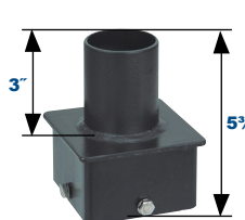
4" Single Square Vertical Tenon - 2 1/2" Dia. PSS43SVTZ
