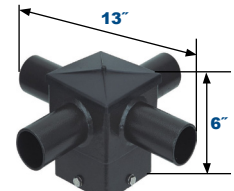
5" 90° Quad Square Horizontal Tenon PSS5Q90HTZ
