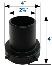
Retrofit Tenon Adaptor for 2 3/8" Tenons PSRTNB
