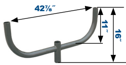
180° Double Bullhorn PRSD180BHZ Wt lbs 17, EPA 0.9
