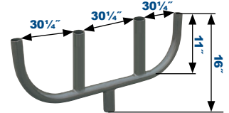
180° Quad Bullhorn PRSQ180BHZ Wt lbs 38, EPA 2.2
