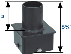
5" Single Square Vertical Tenon - 2 1/4" Dia. PSS53SVTZ
