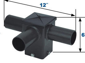
4" 90° Triple Square Horizontal Tenon PSS4TR90HTZ
