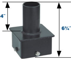
5" Single Square Vertical Tenon - 2 3/8" Dia. PSS52SVTZ
