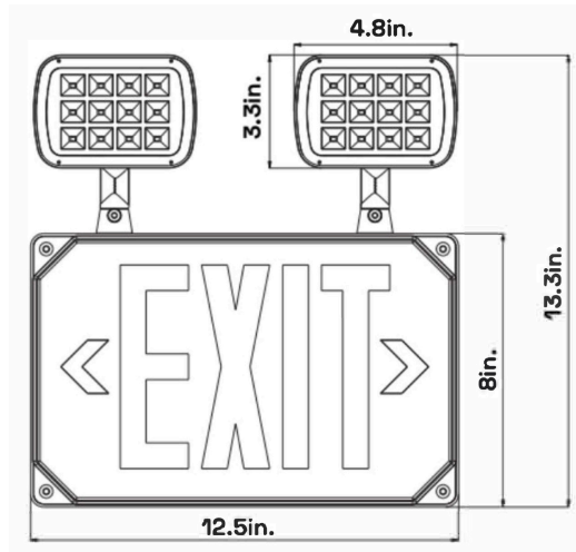
RENATO WET-LOCATION EMERGENCY / EXIT COMBO — FRONT ELEVATION. SIGN BODY 12.50" × 8.00"; EACH HEAD 4.80" × 3.30".
