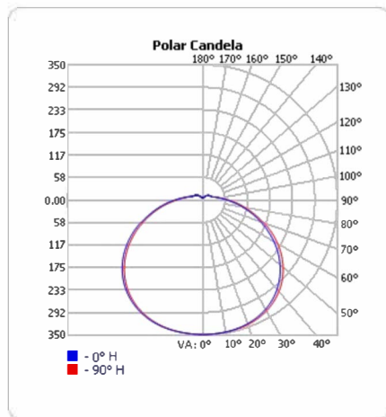
DAWIN 14-20W-5CCT-BN
