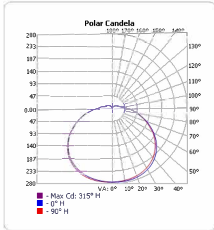
DAWIN 12-16W-5CCT-BN
