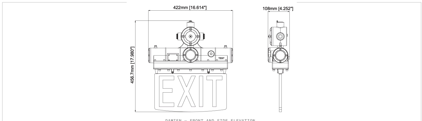
DAMIEN — FRONT AND SIDE ELEVATION.
