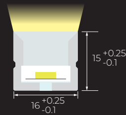
Cross Section(mm)
