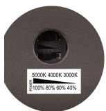
WATT/CCT Selector Switch 4-position power · 3-position CCT
