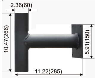
WL Wall Mount Bracket arm
