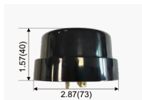
SC Short Cap
