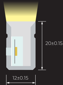
Cross Section(mm)
