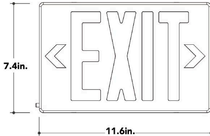
SANCHA COMPACT DOUBLE-SIDED EXIT SIGN — FRONT ELEVATION.
