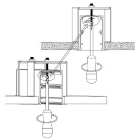
Step 04: Fix the profile
