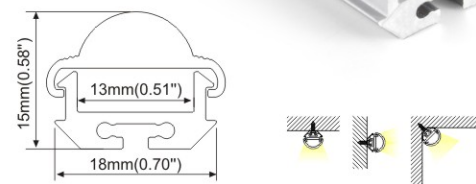
Aluminum profile
