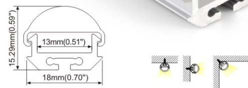
Aluminum profile
