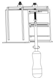
Step 02: Install the recessed frame
