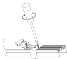
Step 06: Install external clip and the driver
