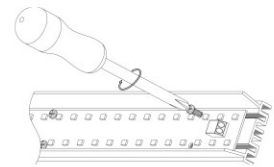
Step 05: Fix the rigid led module
