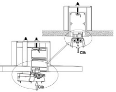
Step 07: Push the gear tray inside the profile
