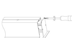
Step 01: Install the end caps
