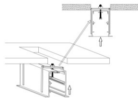
Step 03: Put the whole profile inside the ceiling slot
