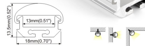
Aluminum profile
