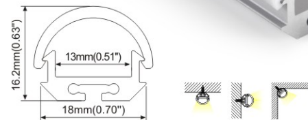
Aluminum profile
