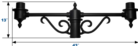
Dual Head Decorative Pole Arm PADAB
