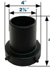
Retrofit Tenon Adaptor for 2 3/8" Tenons PSRTNB
