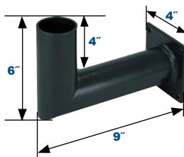
Wall Mount 90° Bracket PRSWMB90Z Wt lbs 4.5, EPA 0.3
