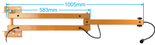
Double Strut Arm (B1 40inch)
