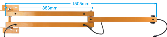
Double Strut Arm (B1 60inch)
