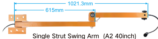
Single Strut Swing Arm (A2 40inch)
