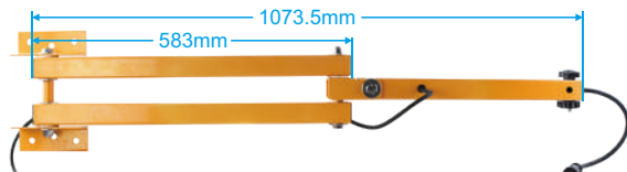
Double Strut Swing Arm (C1 40inch)
